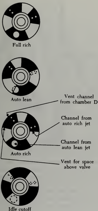
FIGURE 3-20. Manual mixture control valve plate positions.
